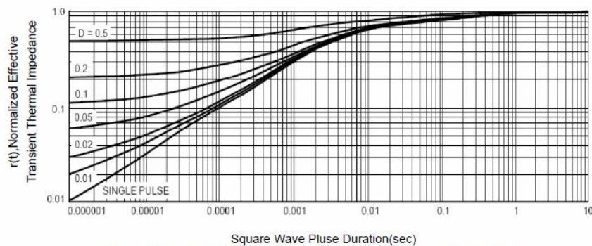
Figure 11 Normalized Maximum Transient Thermal Impedance
