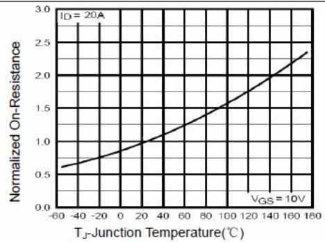
Figure 4 Rds(on)-Junction Temperature
