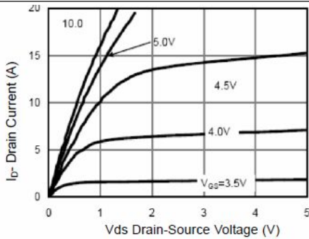
Figure 1 Output Characteristics
