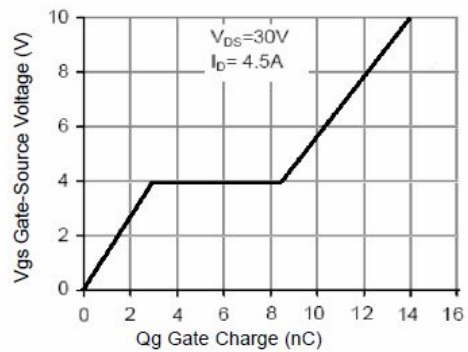
Figure 5 Gate Charge
