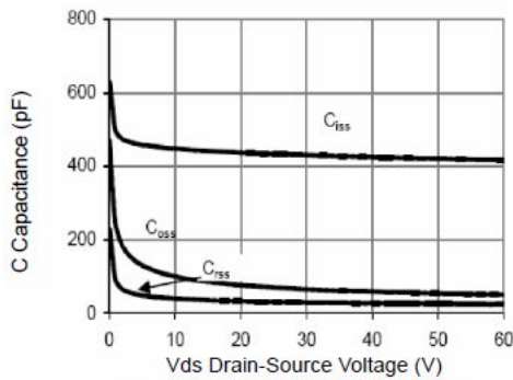
Figure 7 Capacitance vs Vds
